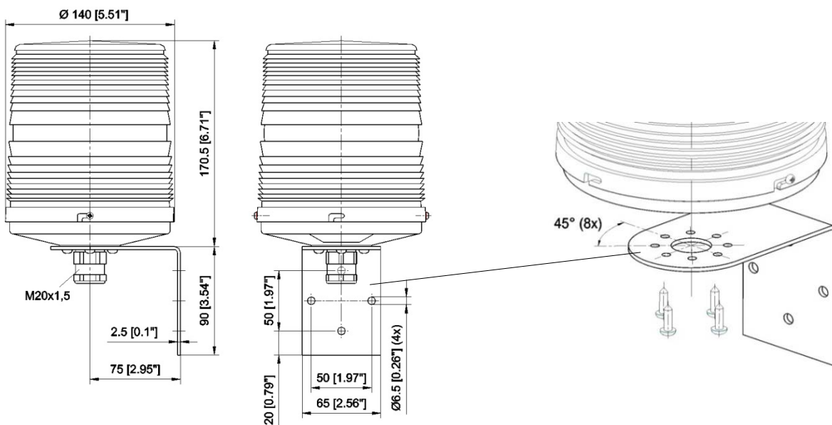
Illustration 6 – Bracket mounting
