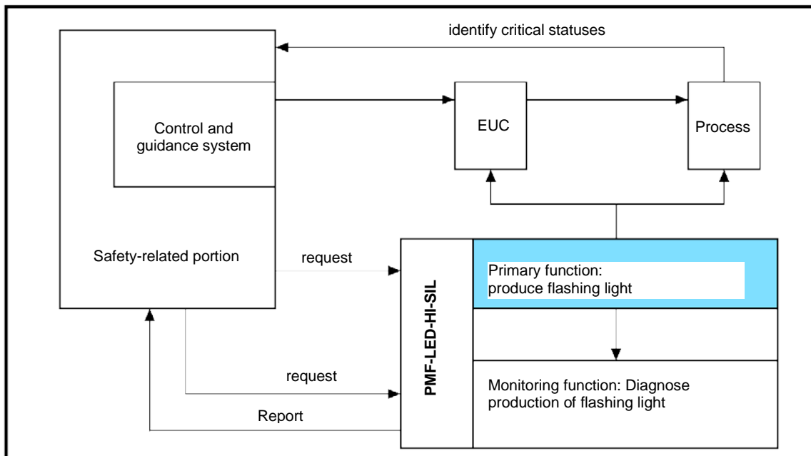
Illustration 4 - Example of a system integration of the monitored warning light
