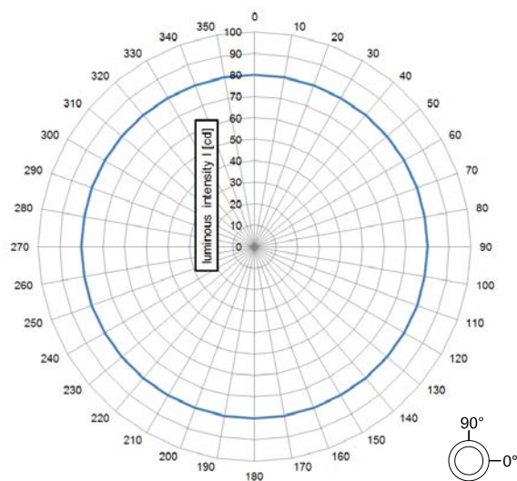
Illustration 1 - Directional diagram
