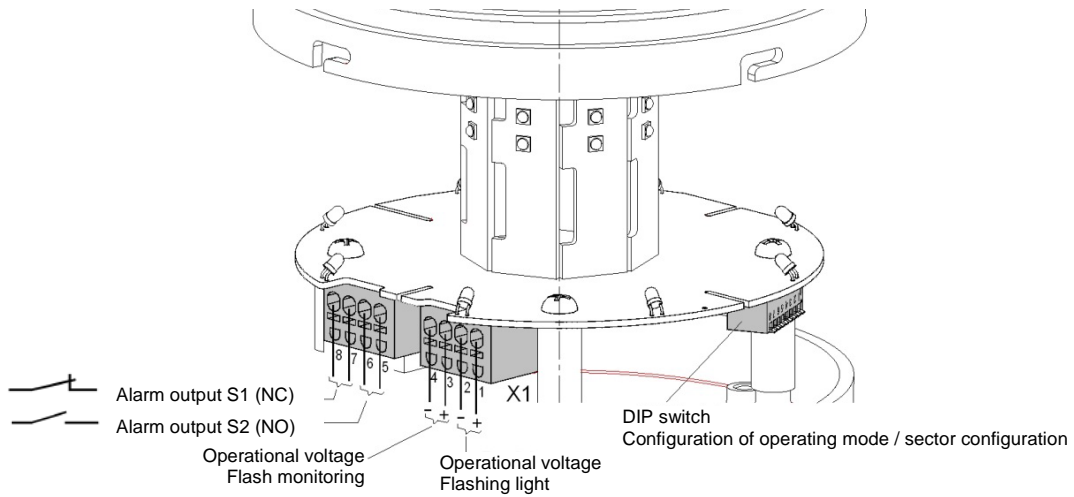
Illustration 8 - Terminal assignment
